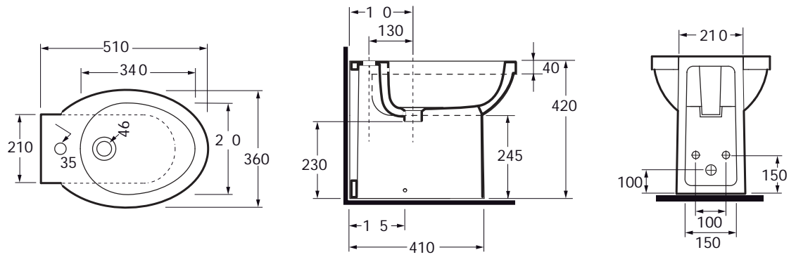
Art. SPBT3 Bidet a terra Back to wall bidet
